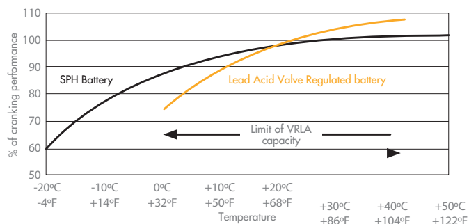
SPH versus Valve Regulated Lead Acid: variation of cranking performance according to temperature
