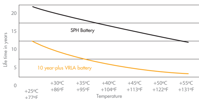
SPH versus Valve Regulated Lead Acid: variation of lifetime according to temperature
