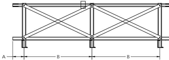
7' - 10' RACKS (3 FRAMES)
