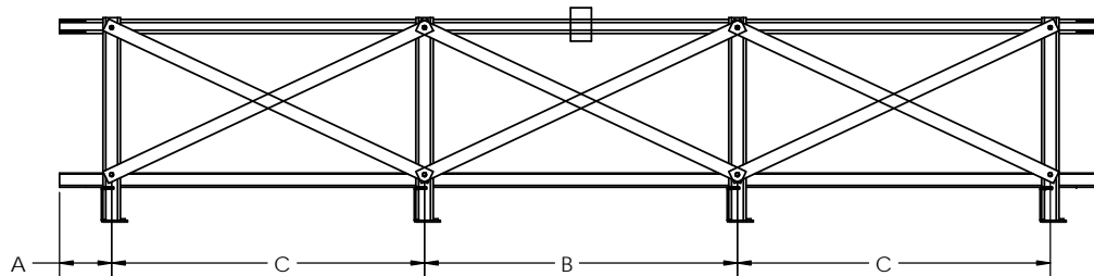
11' - 14' RACKS (4 FRAMES)
