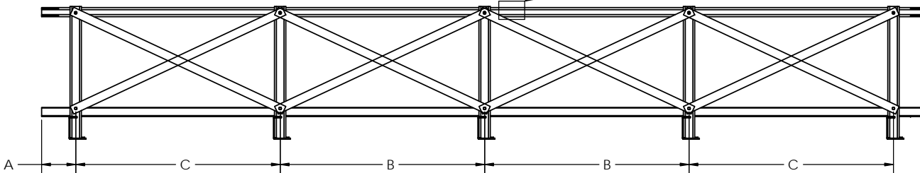
15' - 18' RACKS (5 FRAMES)
