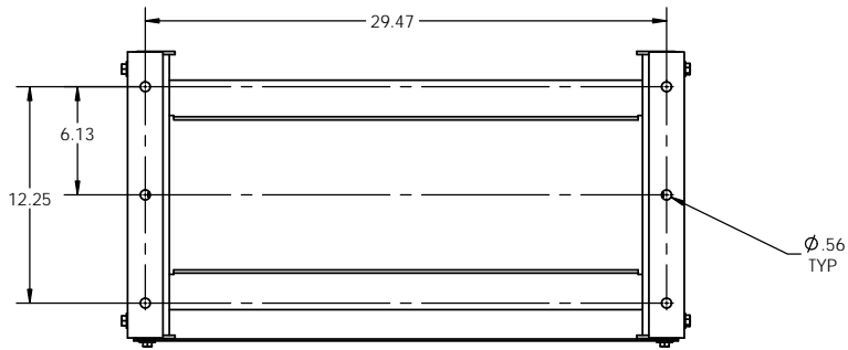
BOTTOM VIEW OPTIONAL SEISMIC MOUNTING FOOTPRINT
